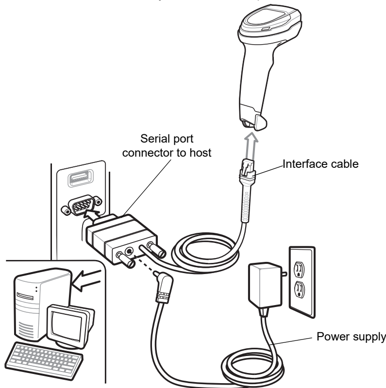
Figure 7-1 RS-232 Connection
